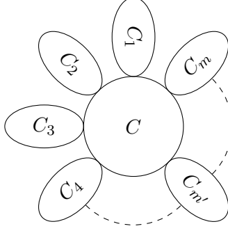
Figure 1: A sunflower with m petals.
