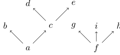
Figure 2: The forest in Example 11
