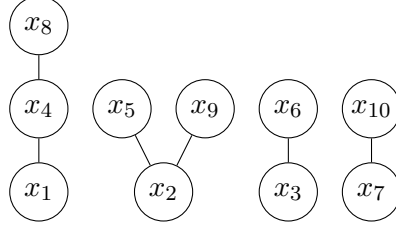
Figure 3: The complement graph G(I) of the instance I in Example 21.
