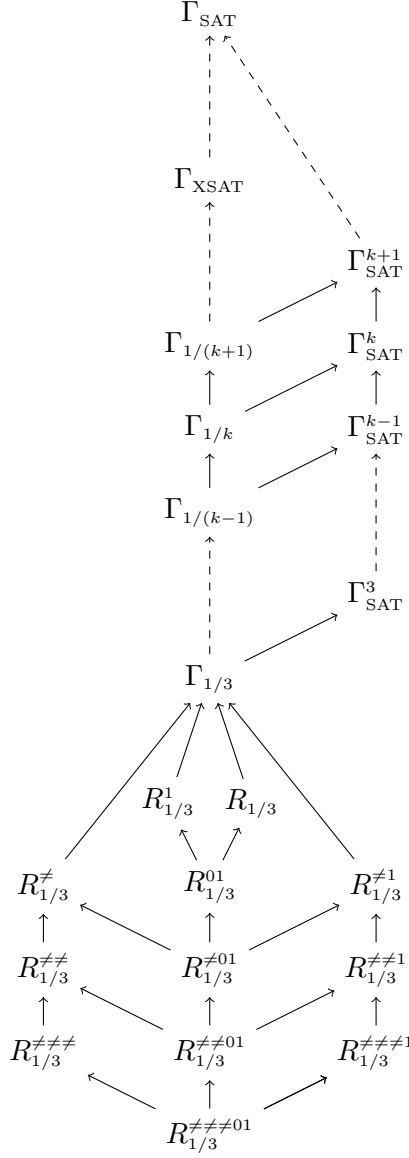
Figure 4: The structure of some partial co-clones in \mathcal{I}(\text{BR}) . A directed arrow from S to S' means \langle S \rangle_{\overline{\mathcal{F}}} \subset \langle S' \rangle_{\overline{\mathcal{F}}} and hence also \mathbb{T}(S) \leq \mathbb{T}(S') . Some trivial inclusions, for example that every node \Gamma satisfies \langle \Gamma \rangle_{\overline{\mathcal{F}}} \subseteq \langle \Gamma_{\text{SAT}} \rangle_{\overline{\mathcal{F}}} , have been omitted in the figure.
