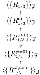
Figure 1: The conjectured structure of weak partial co-clones below \langle \{R_{1/3}\} \rangle_{\neq} . A directed arrow A \rightarrow B means that A \subset B .
