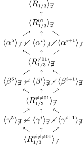
Figure 2: The structure of weak partial co-clones below \langle R_{1/3} \rangle_{\exists} . An arrow of the form A \rightarrow B means that A \subset B . An arrow of the form A \not\rightarrow B means that A \not\subset B .
